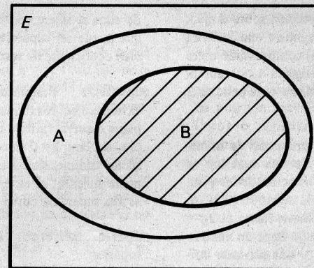
B \subset A
